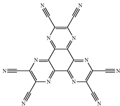
HATCN
